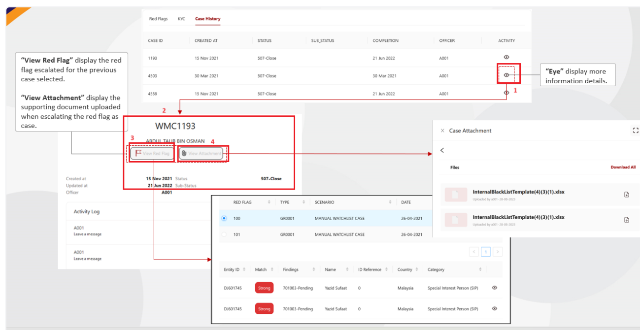
Figure 2.14: Case History Process Flow
