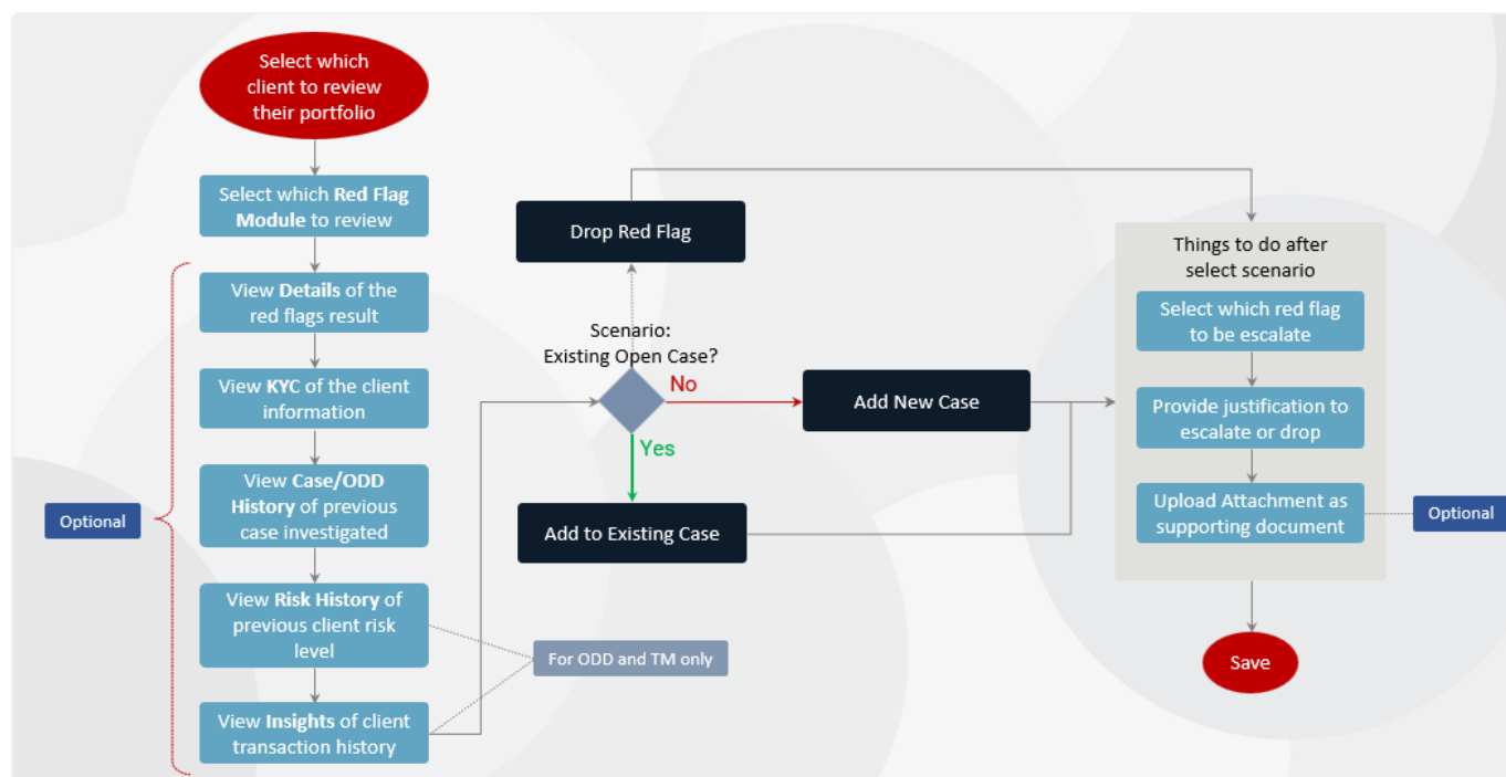
Figure 2.25: App Process Flow to Manage Transaction Monitoring (TM) Red Flag
