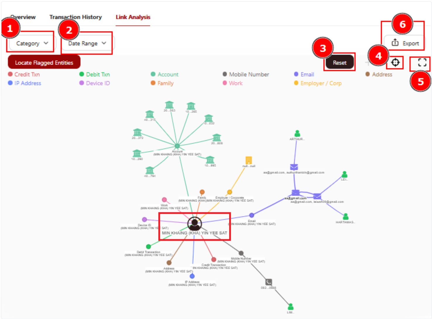
Figure 2.23: Link Analysis condition node
